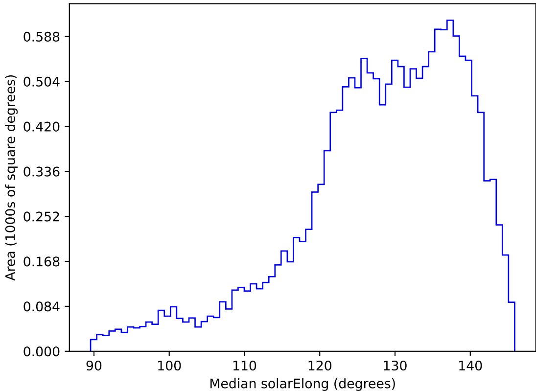
ddf_acor_sf15_lsf40_lsr20_v3.4_10yrs WFD z band: Median solarElong
