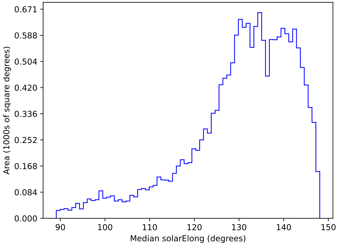
ddf_acor_sf15_lsf40_lsr20_v3.4_10yrs WFD r band: Median solarElong
