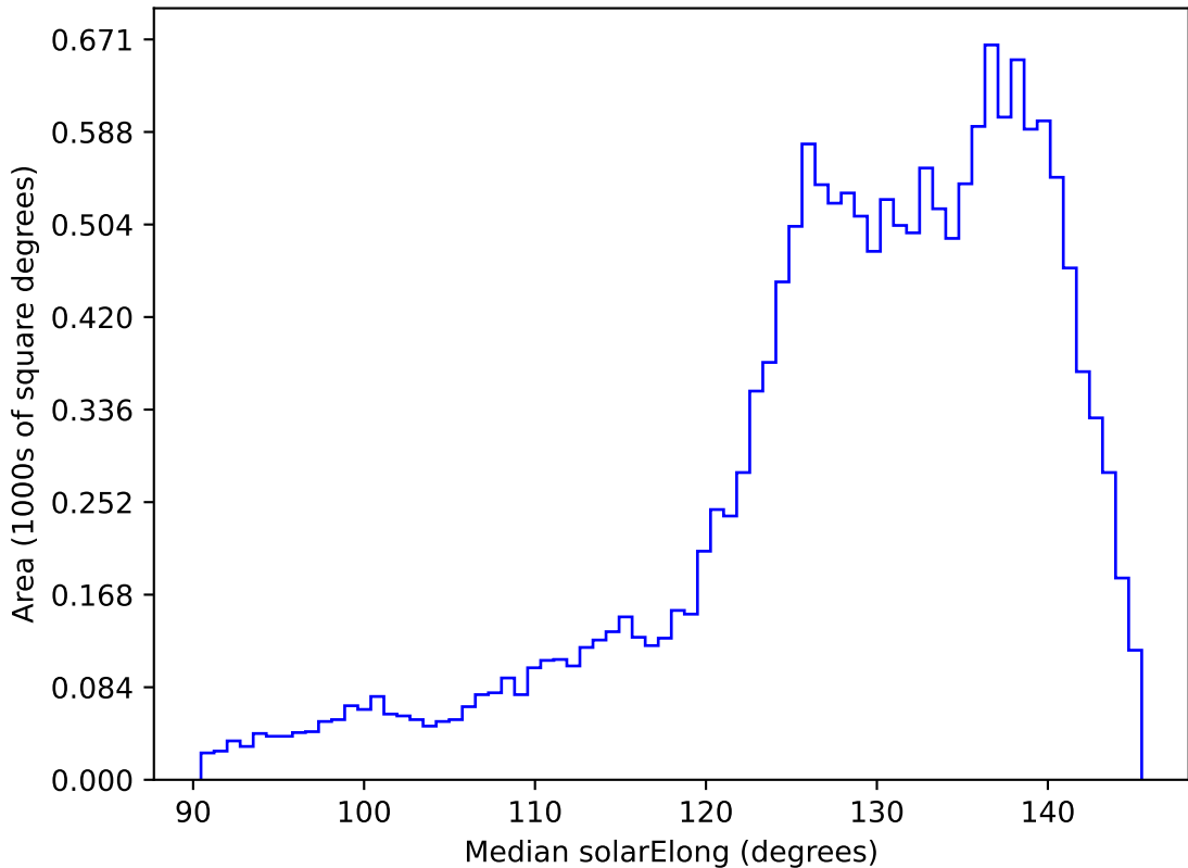
ddf_acor_sf15_lsf40_lsr20_v3.4_10yrs WFD i band: Median solarElong
