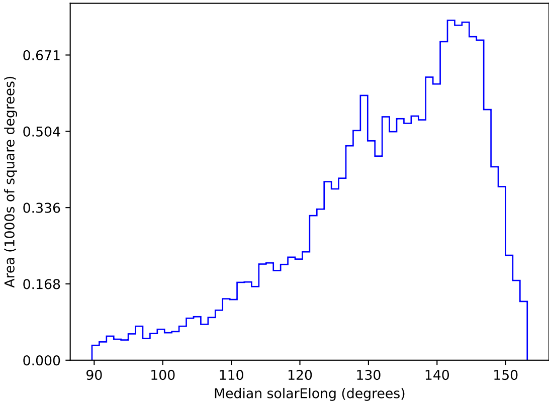
ddf_acor_sf15_lsf40_lsr20_v3.4_10yrs WFD g band: Median solarElong
