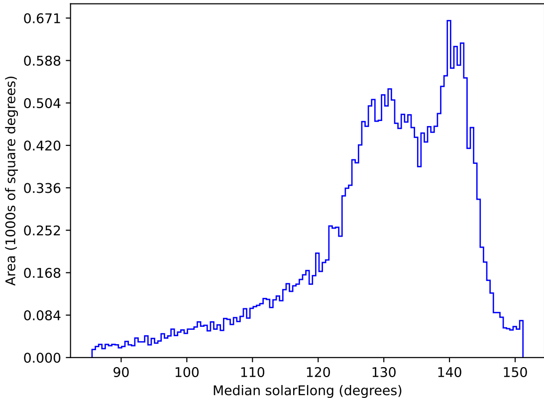
ddf_acor_sf15_lsf40_lsr20_v3.4_10yrs All sky all bands: Median solarElong
