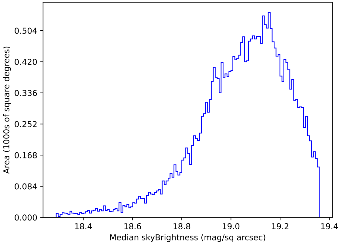
ddf_acor_sf15_lsf40_lsr20_v3.4_10yrs Yr 1 z band: Median skyBrightness
