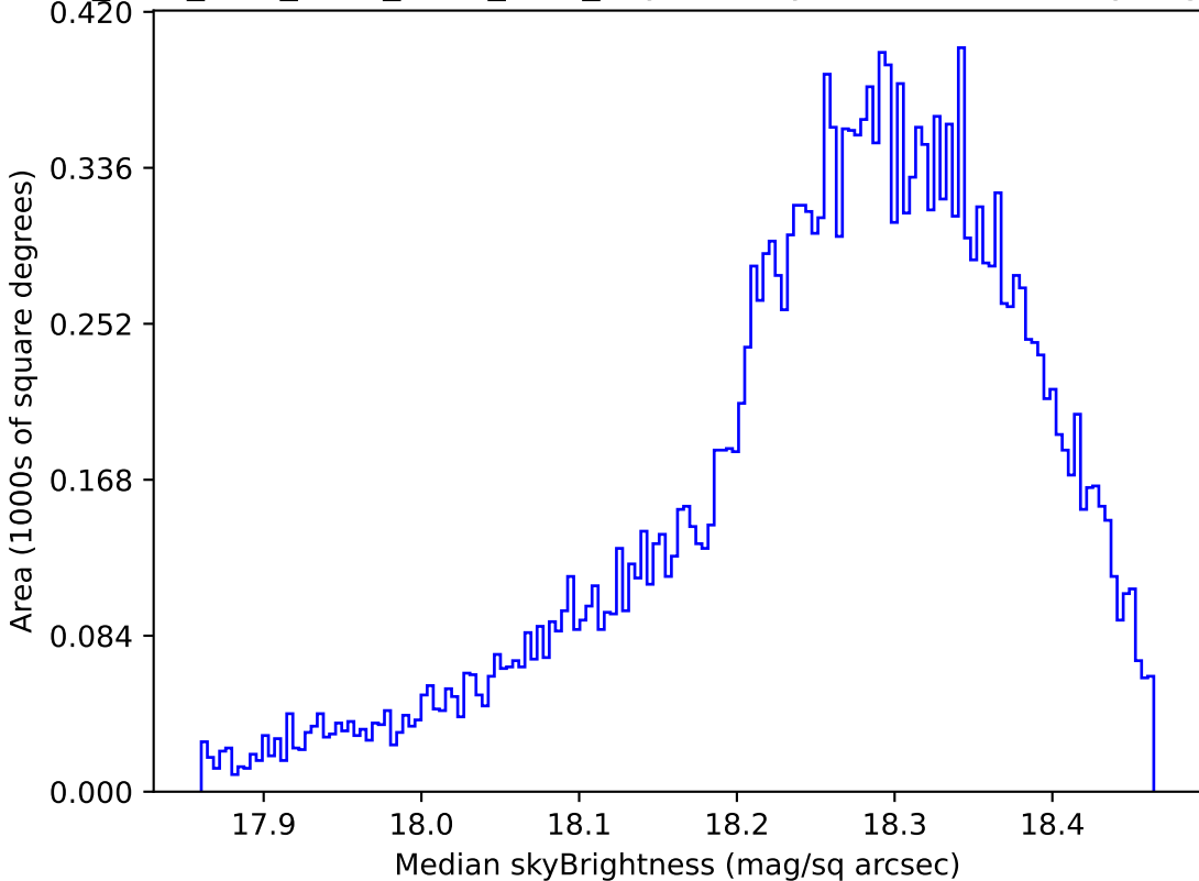
ddf_acor_sf15_Isf40_Isr20_v3.4_10yrs Yr 1 y band: Median skyBrightness
