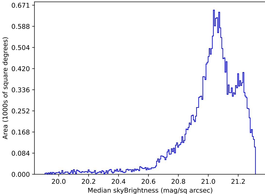
ddf_acor_sf15_lsf40_lsr20_v3.4_10yrs Yr 1 r band: Median skyBrightness
