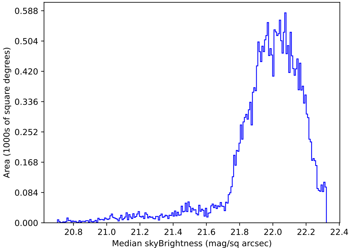
ddf_acor_sf15_lsf40_lsr20_v3.4_10yrs Yr 1 g band: Median skyBrightness
