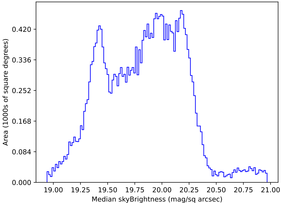
ddf_acor_sf15_lsf40_lsr20_v3.4_10yrs Yr 1 all bands: Median skyBrightness
