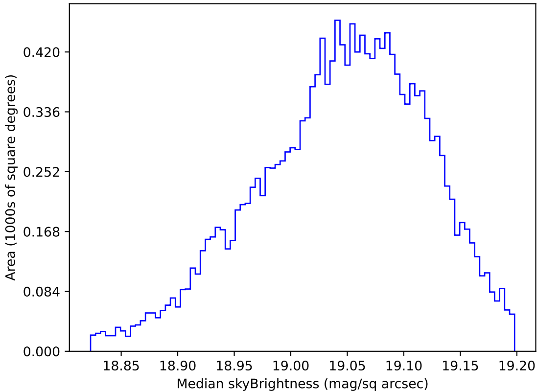
ddf_acor_sf15_lsf40_lsr20_v3.4_10yrs WFD z band: Median skyBrightness
