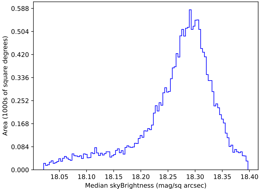
ddf_acor_sf15_lsf40_lsr20_v3.4_10yrs WFD y band: Median skyBrightness
