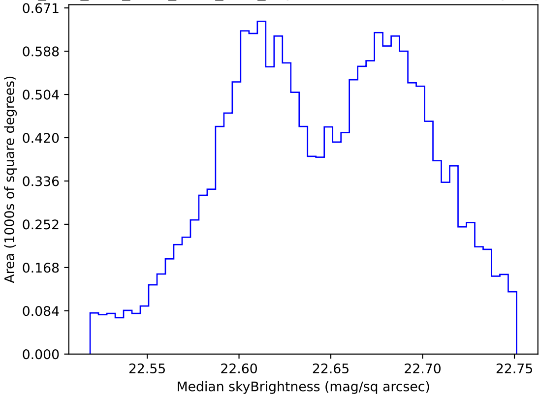
ddf_acor_sf15_lsf40_lsr20_v3.4_10yrs WFD u band: Median skyBrightness
