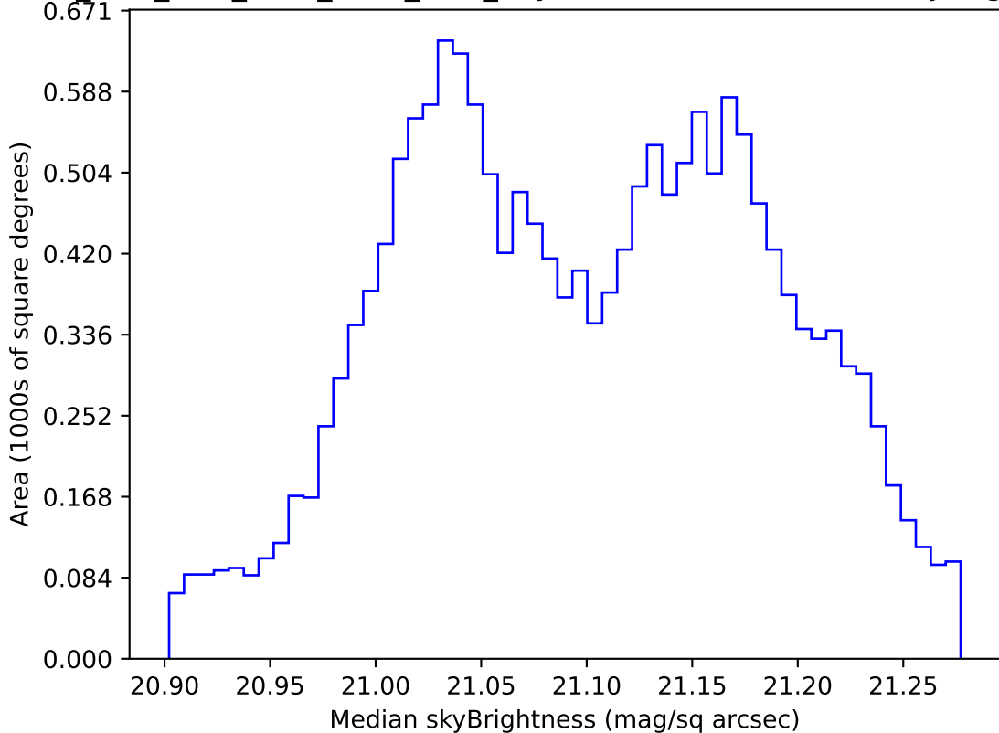
ddf_acor_sf15_lsf40_lsr20_v3.4_10yrs WFD r band: Median skyBrightness
