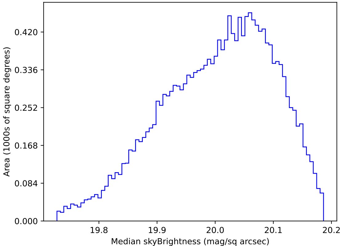
ddf_acor_sf15_lsf40_lsr20_v3.4_10yrs WFD i band: Median skyBrightness
