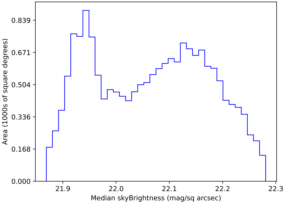
ddf_acor_sf15_lsf40_lsr20_v3.4_10yrs WFD g band: Median skyBrightness
