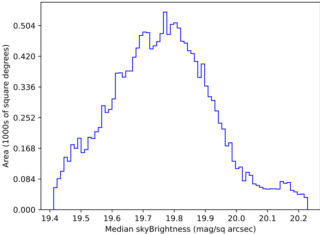
ddf_acor_sf15_lsf40_lsr20_v3.4_10yrs WFD all bands: Median skyBrightness
