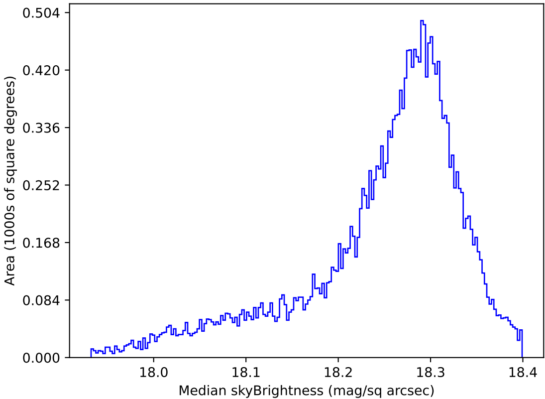
ddf_acor_sf15_lsf40_lsr20_v3.4_10yrs All sky y band: Median skyBrightness
