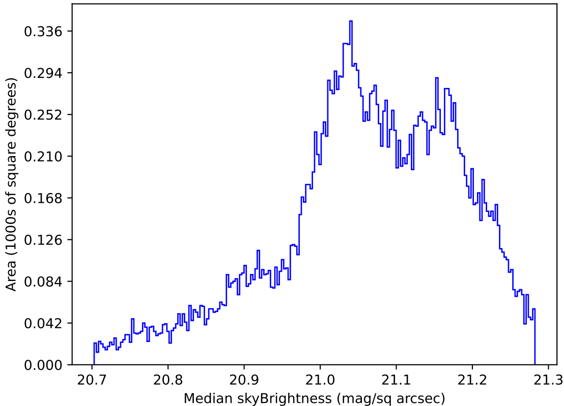
ddf_acor_sf15_lsf40_lsr20_v3.4_10yrs All sky r band: Median skyBrightness
