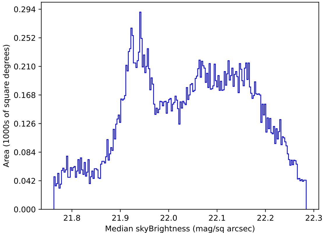
ddf_acor_sf15_lsf40_lsr20_v3.4_10yrs All sky g band: Median skyBrightness
