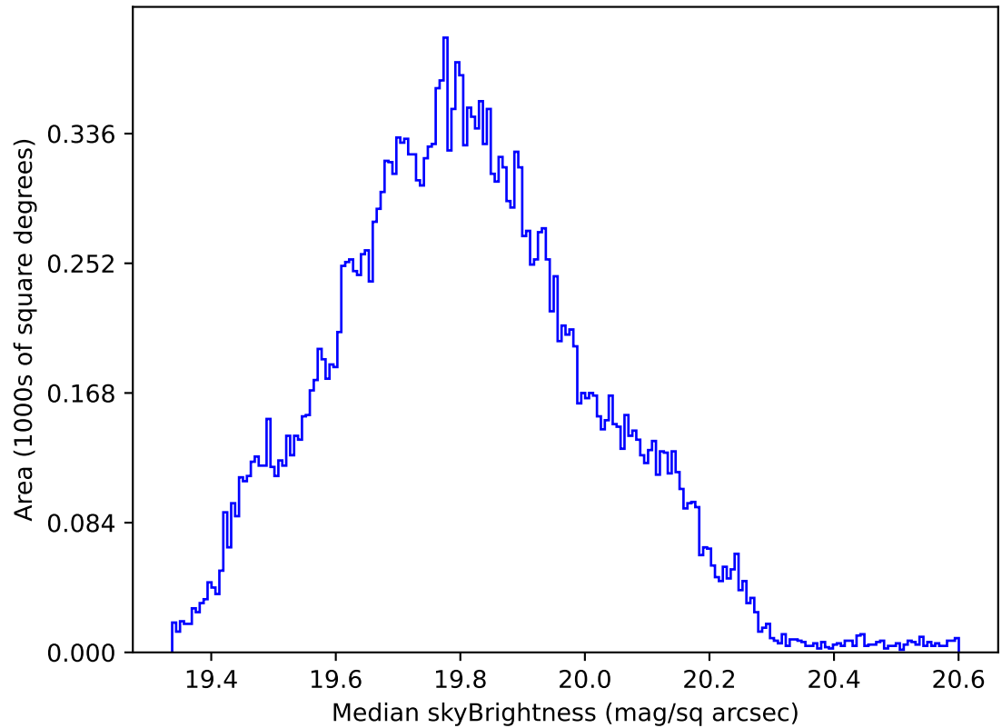
ddf_acor_sf15_lsf40_lsr20_v3.4_10yrs All sky all bands: Median skyBrightness
