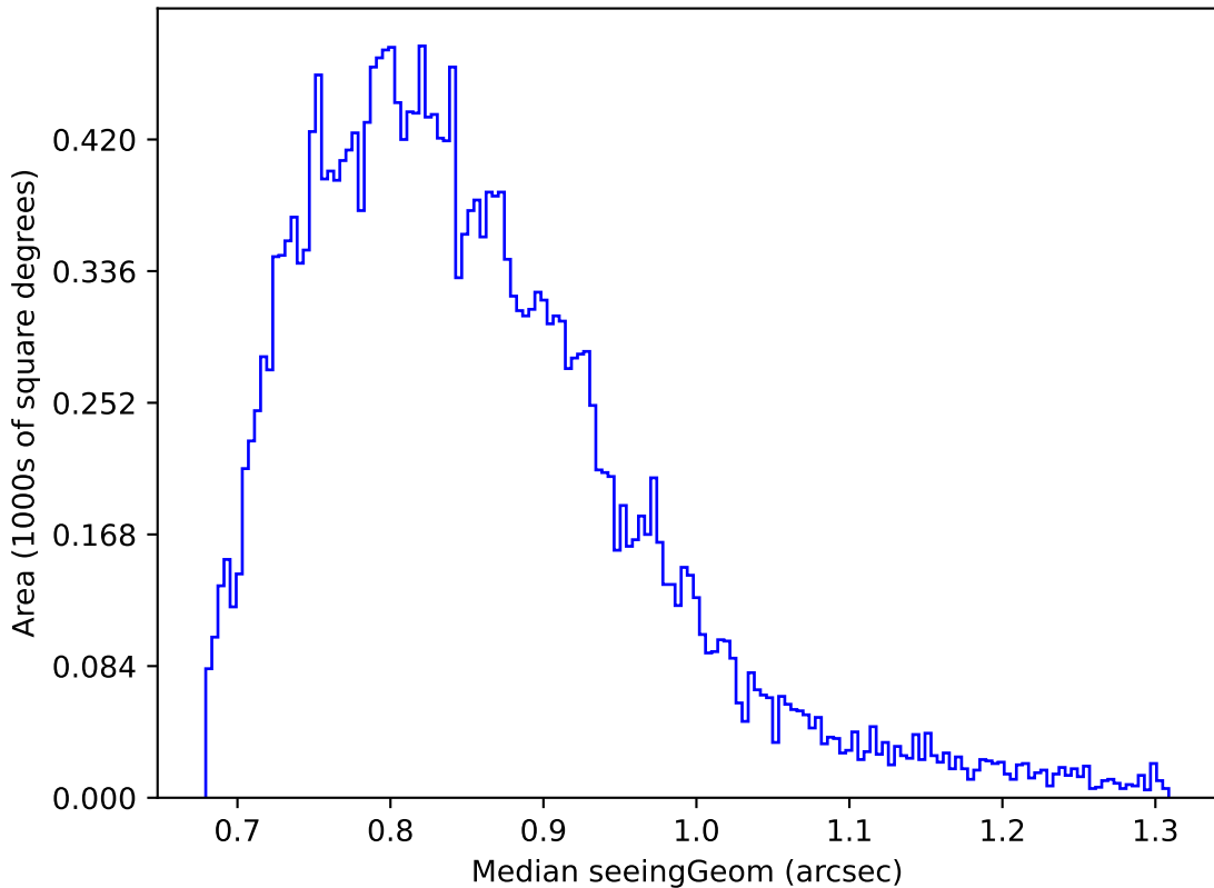
ddf_acor_sf15_lsf40_lsr20_v3.4_10yrs Yr 1 z band: Median seeingGeom
