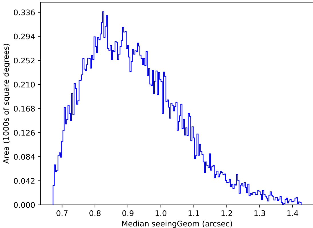
ddf_acor_sf15_lsf40_lsr20_v3.4_10yrs Yr 1 g band: Median seeingGeom
