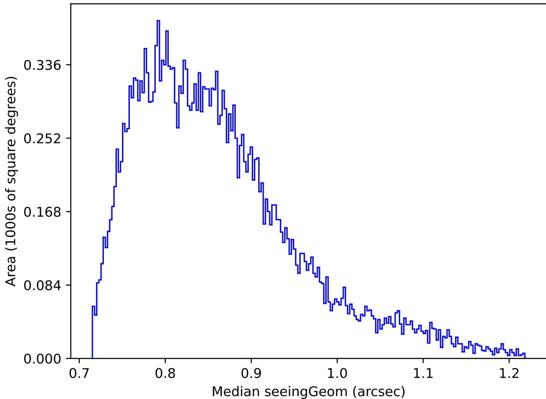
ddf_acor_sf15_lsf40_lsr20_v3.4_10yrs Yr 1 all bands: Median seeingGeom
