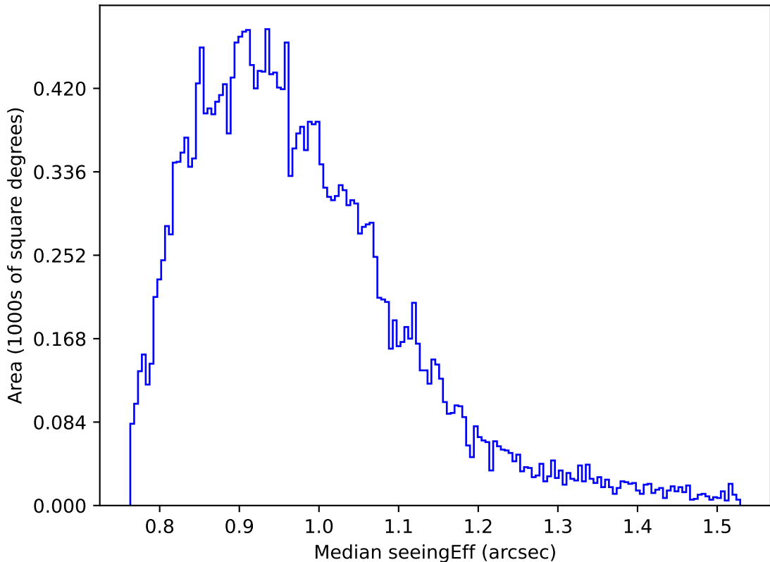
ddf_acor_sf15_lsf40_lsr20_v3.4_10yrs Yr 1 z band: Median seeingEff
