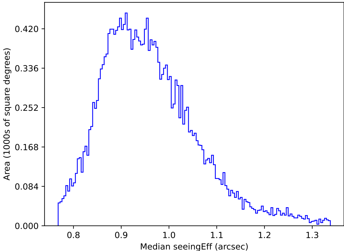
ddf_acor_sf15_lsf40_lsr20_v3.4_10yrs Yr 1 y band: Median seeingEff
