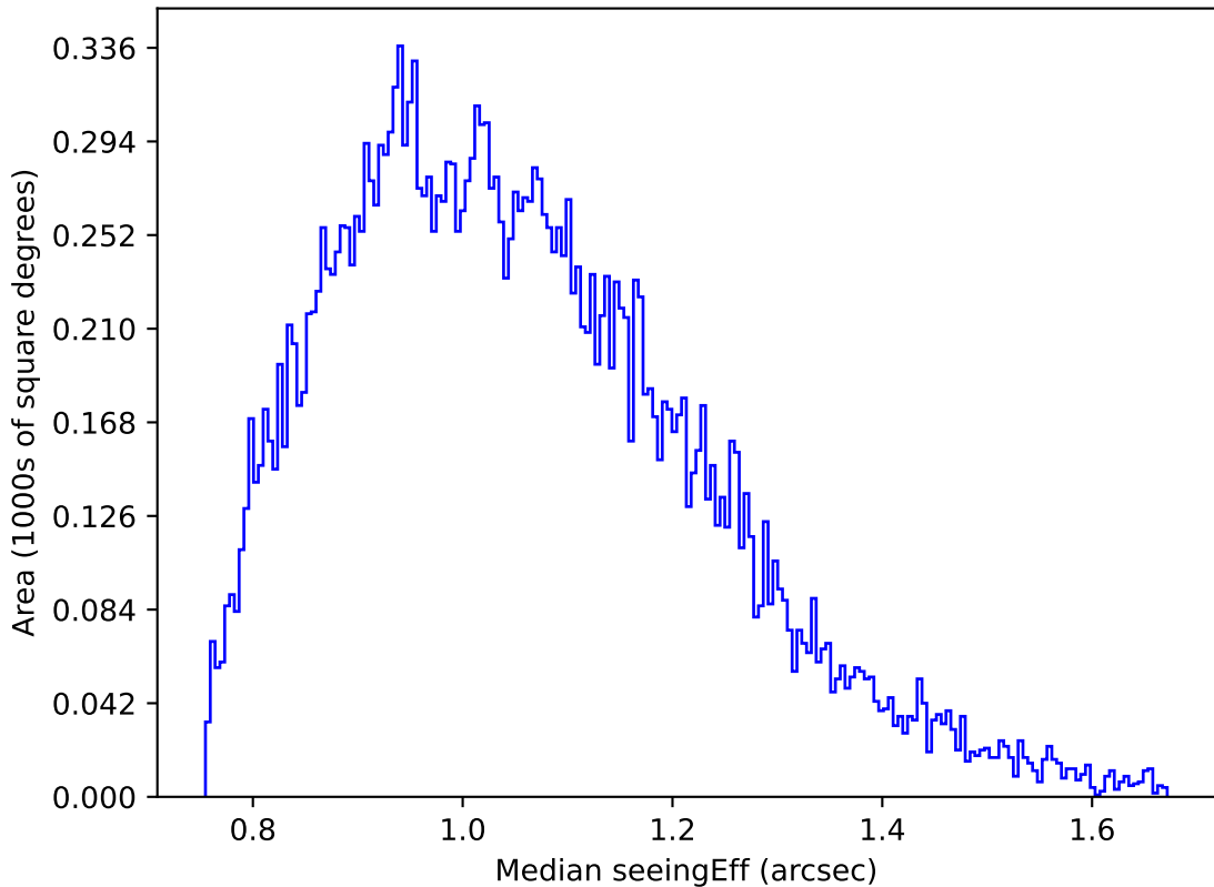
ddf_acor_sf15_lsf40_lsr20_v3.4_10yrs Yr 1 g band: Median seeingEff
