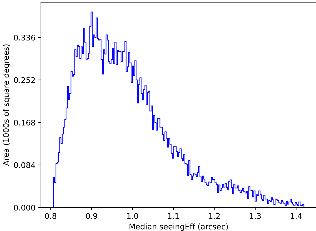
ddf_acor_sf15_lsf40_lsr20_v3.4_10yrs Yr 1 all bands: Median seeingEff
