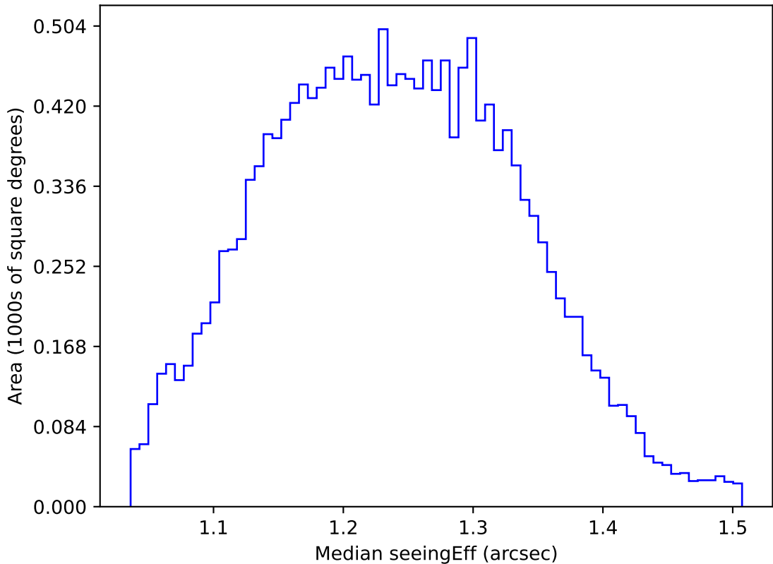
ddf_acor_sf15_lsf40_lsr20_v3.4_10yrs WFD u band: Median seeingEff
