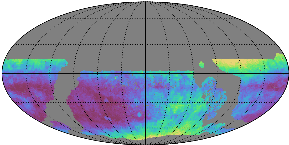
ddf_acor_sf15_lsf40_lsr20_v3.4_10yrs WFD i band: Median seeingEff
