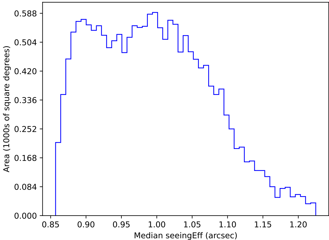
ddf_acor_sf15_lsf40_lsr20_v3.4_10yrs WFD i band: Median seeingEff
