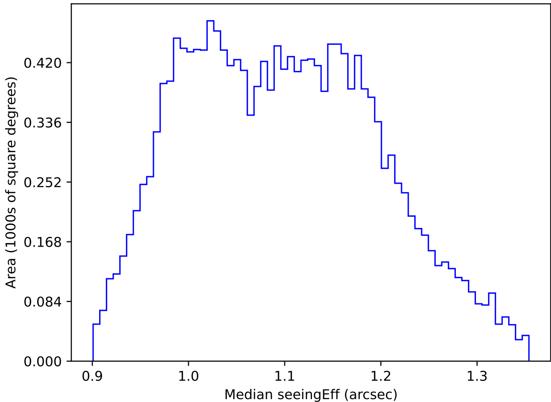
ddf_acor_sf15_lsf40_lsr20_v3.4_10yrs WFD g band: Median seeingEff
