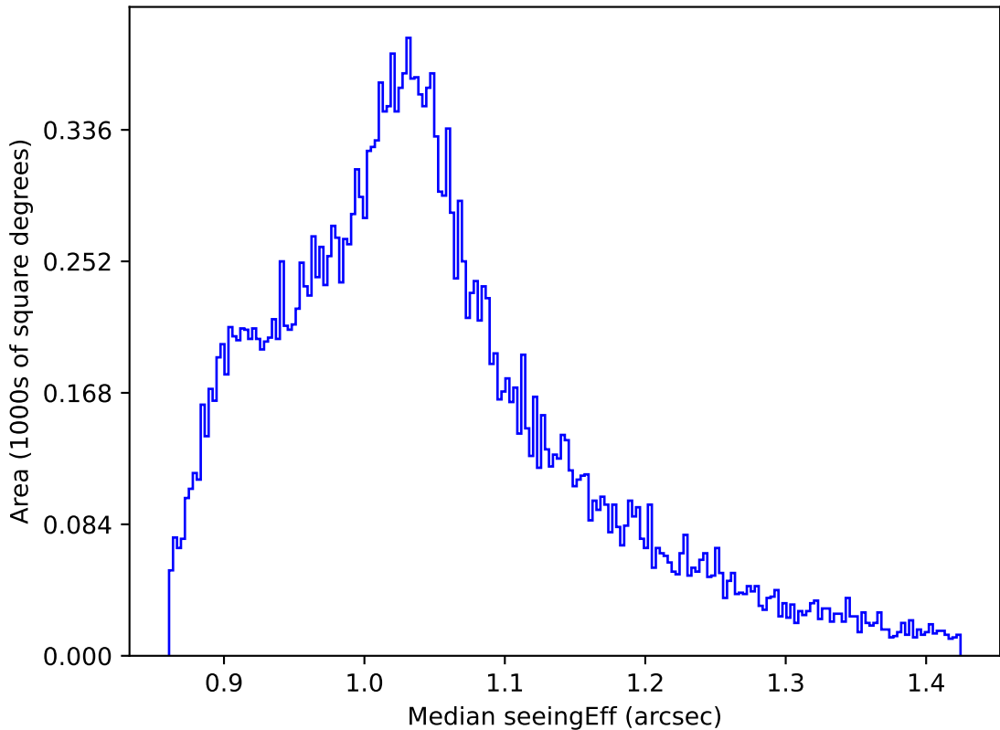
ddf_acor_sf15_lsf40_lsr20_v3.4_10yrs All sky z band: Median seeingEff
