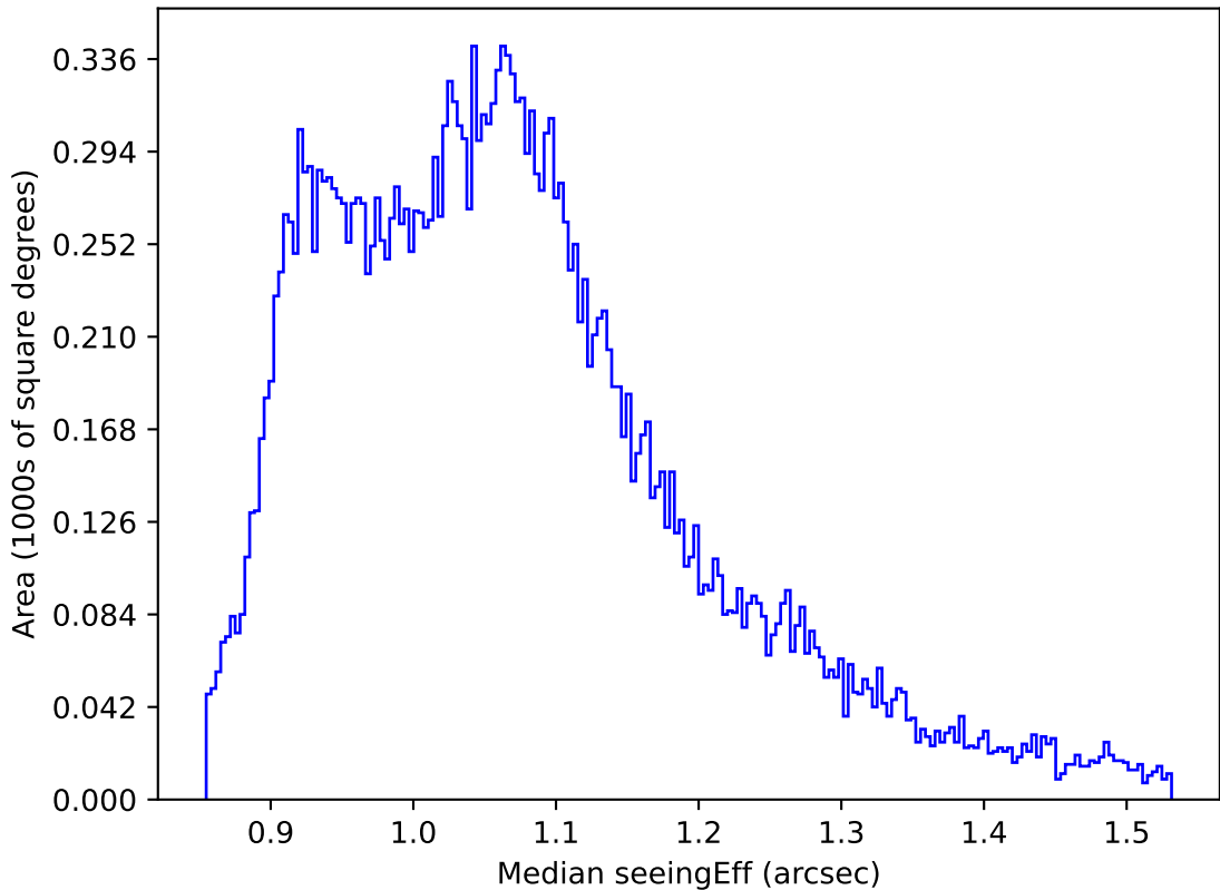
ddf_acor_sf15_lsf40_lsr20_v3.4_10yrs All sky r band: Median seeingEff
