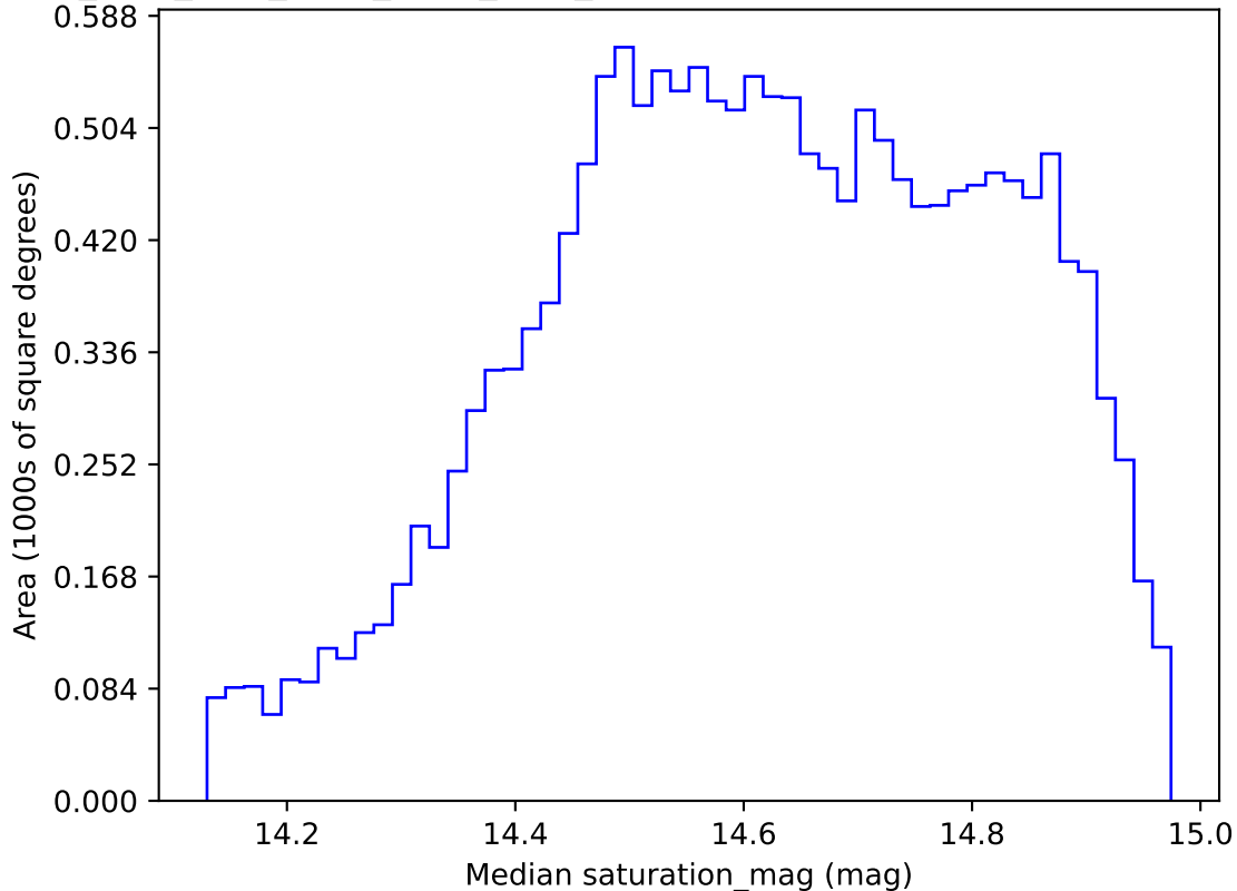
ddf_acor_sf15_lsf40_lsr20_v3.4_10yrs WFD r band: Median saturation_mag
