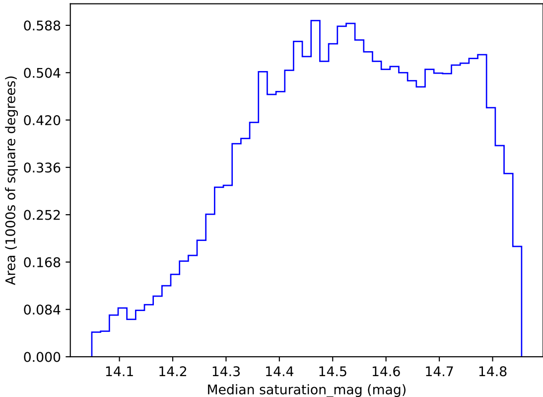
ddf_acor_sf15_lsf40_lsr20_v3.4_10yrs WFD i band: Median saturation_mag
