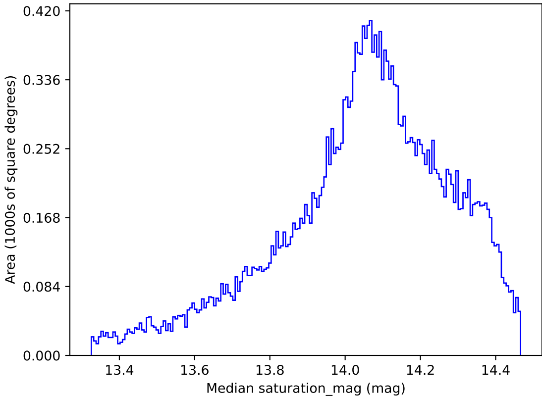
ddf_acor_sf15_lsf40_lsr20_v3.4_10yrs All sky z band: Median saturation_mag
