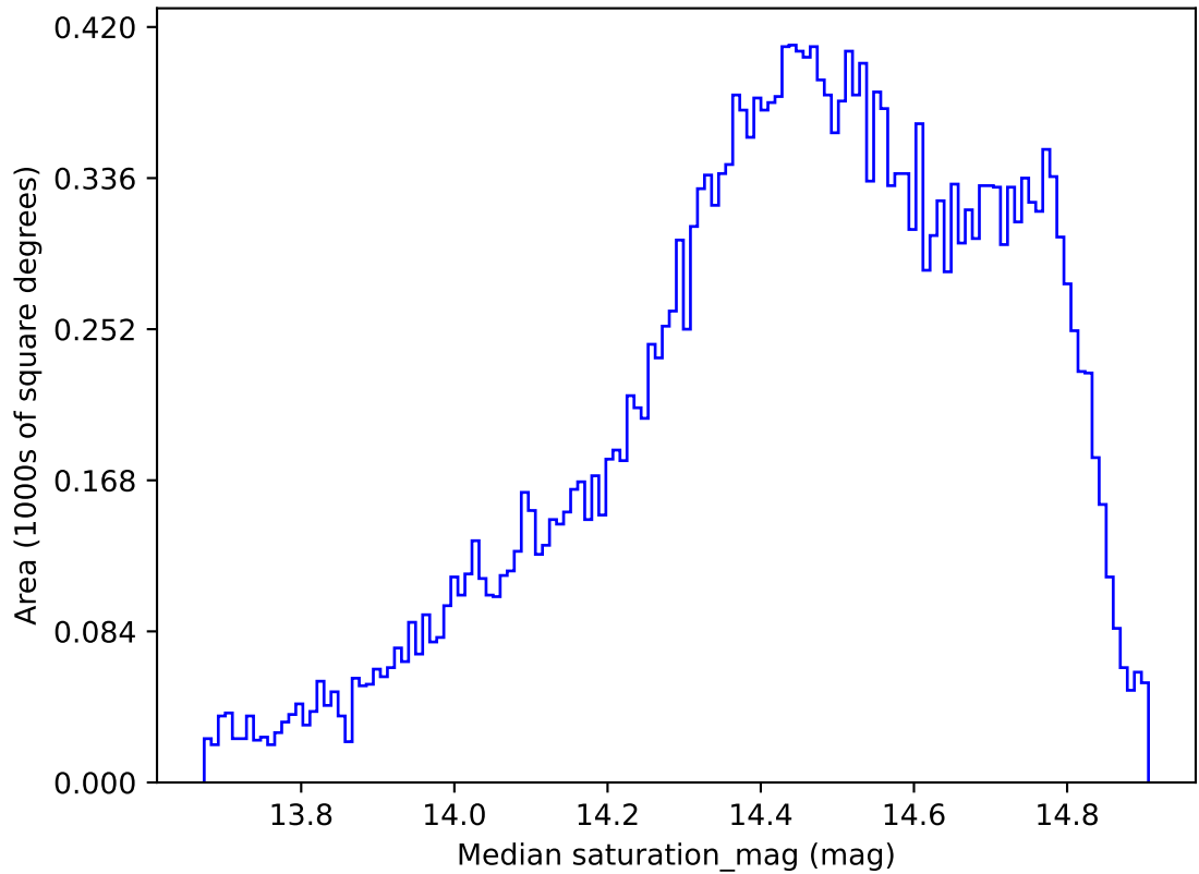
ddf_acor_sf15_lsf40_lsr20_v3.4_10yrs All sky i band: Median saturation_mag
