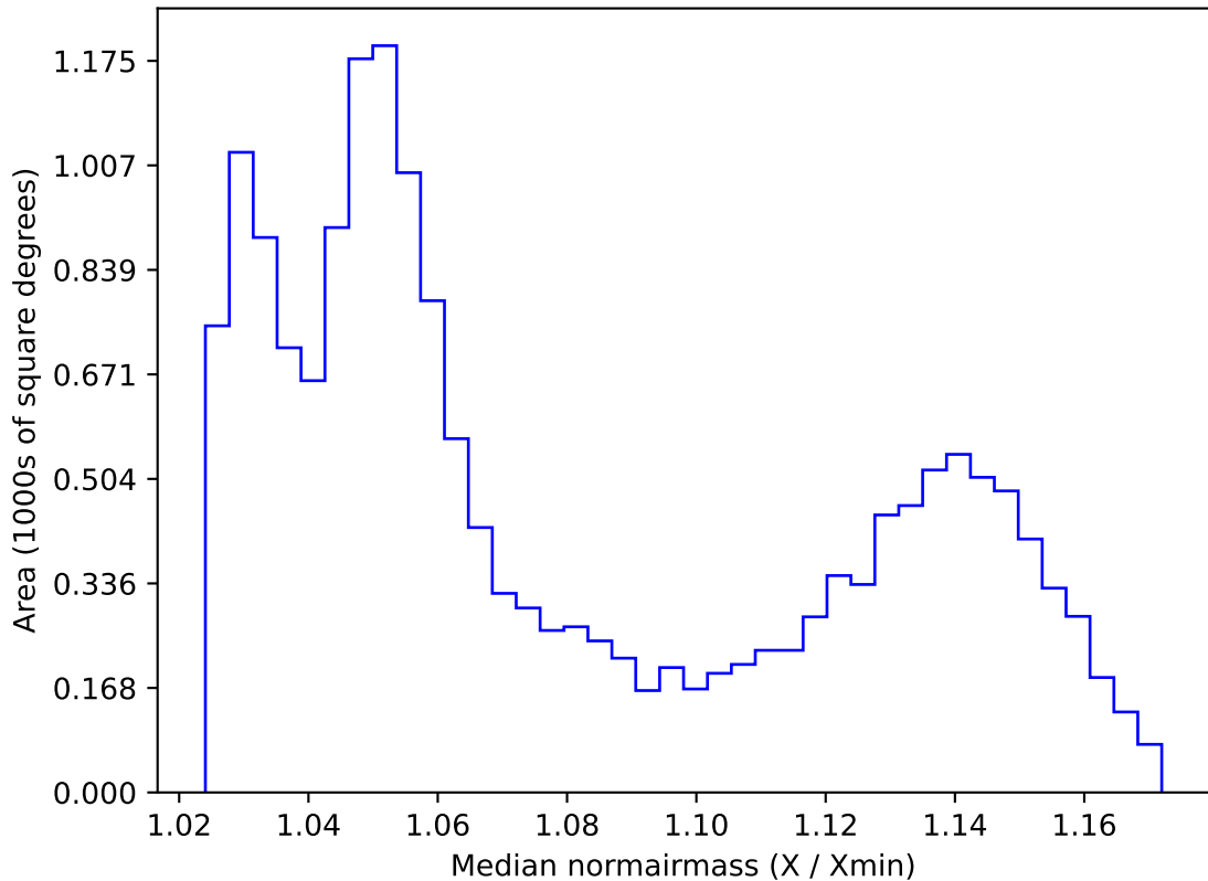
ddf_acor_sf15_lsf40_lsr20_v3.4_10yrs WFD all bands: Median normairmass
