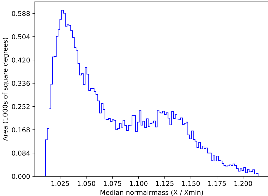
ddf_acor_sf15_lsf40_lsr20_v3.4_10yrs All sky u band: Median normairmass
