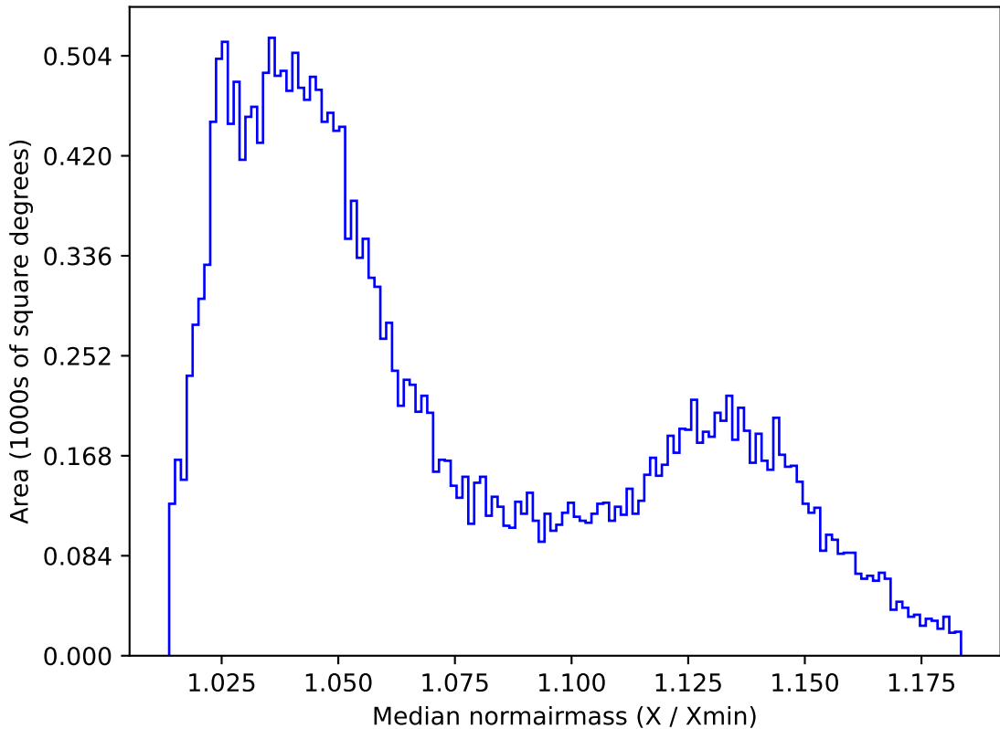
ddf_acor_sf15_lsf40_lsr20_v3.4_10yrs All sky r band: Median normairmass
