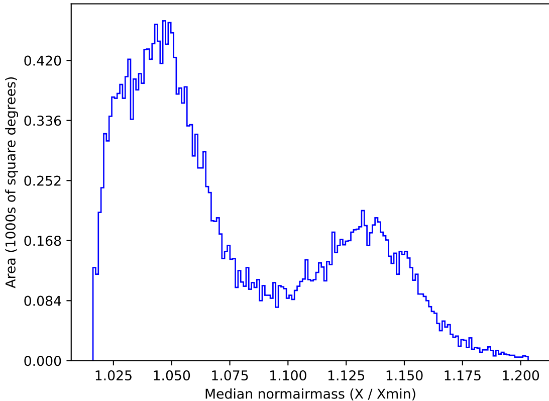
ddf_acor_sf15_lsf40_lsr20_v3.4_10yrs All sky i band: Median normairmass
