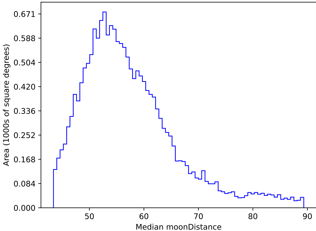
ddf_acor_sf15_lsf40_lsr20_v3.4_10yrs WFD y band: Median moonDistance
