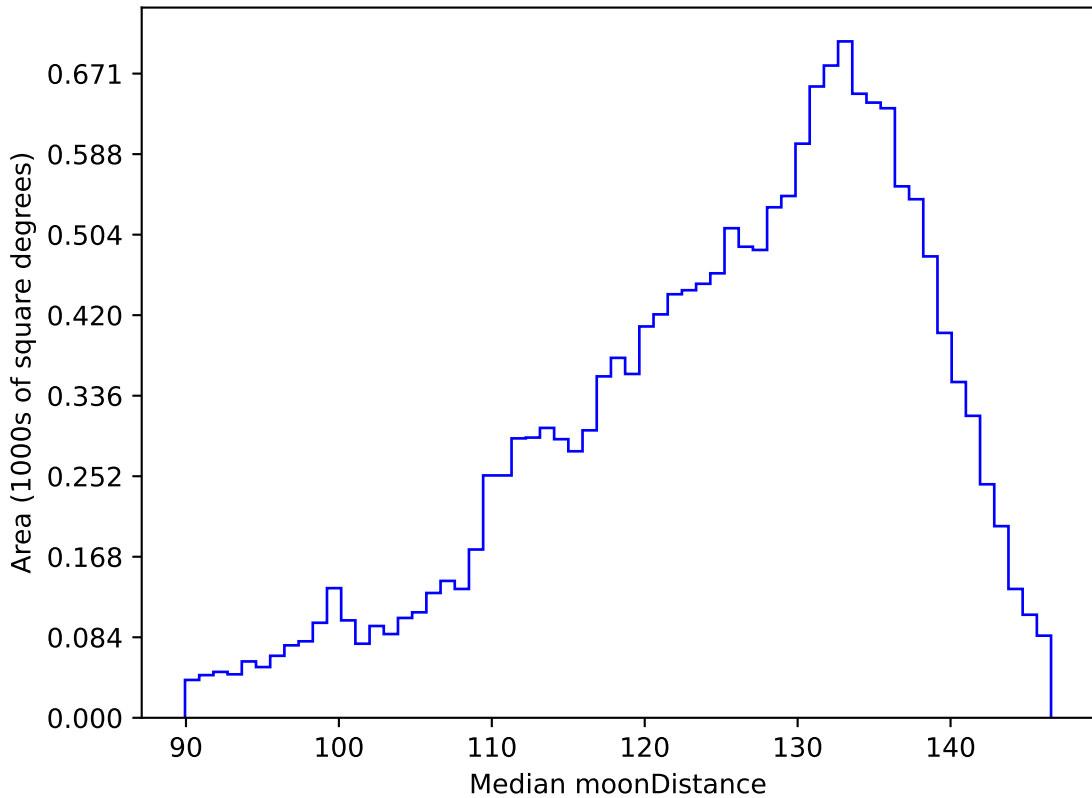
ddf_acor_sf15_lsf40_lsr20_v3.4_10yrs WFD u band: Median moonDistance
