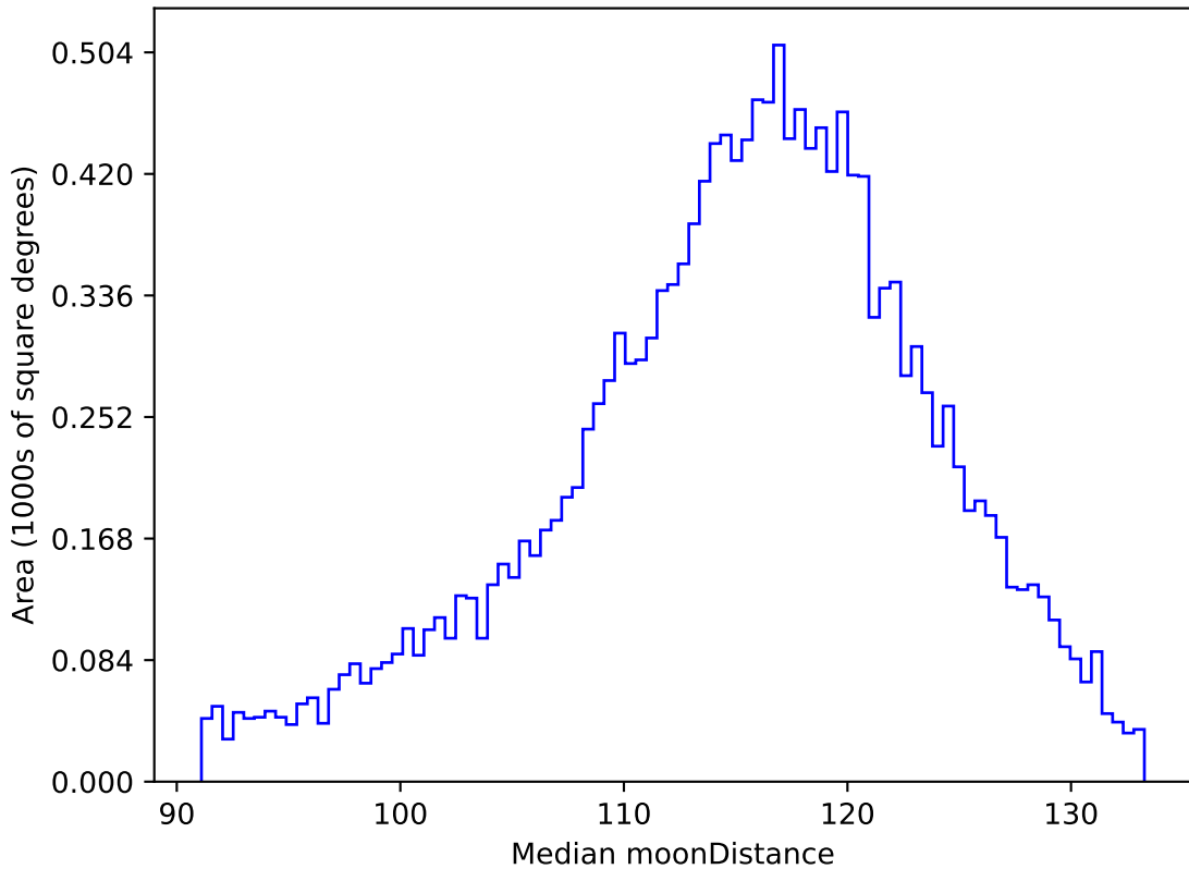
ddf_acor_sf15_lsf40_lsr20_v3.4_10yrs WFD g band: Median moonDistance
