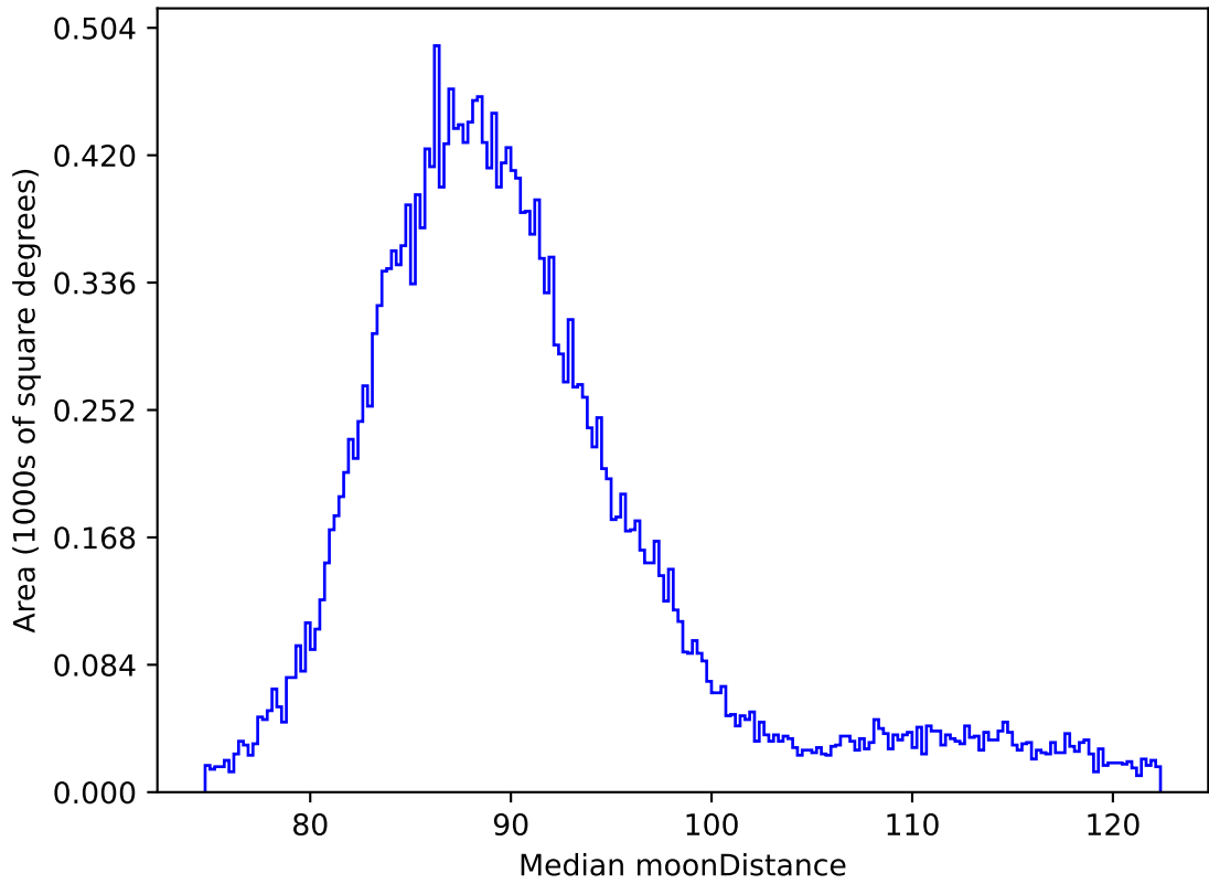
ddf_acor_sf15_lsf40_lsr20_v3.4_10yrs All sky all bands: Median moonDistance
