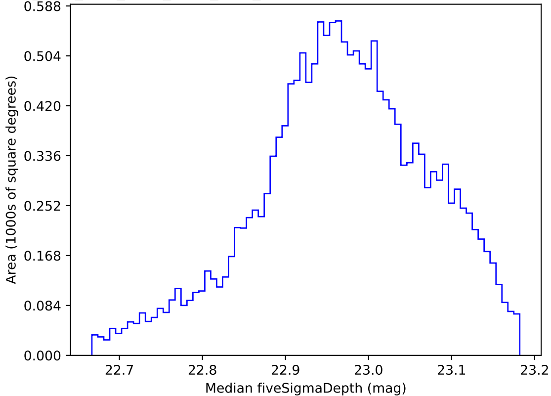
ddf_acor_sf15_ls40_lsr20_v3.4_10yrs WFD z band: Median fiveSigmaDepth
