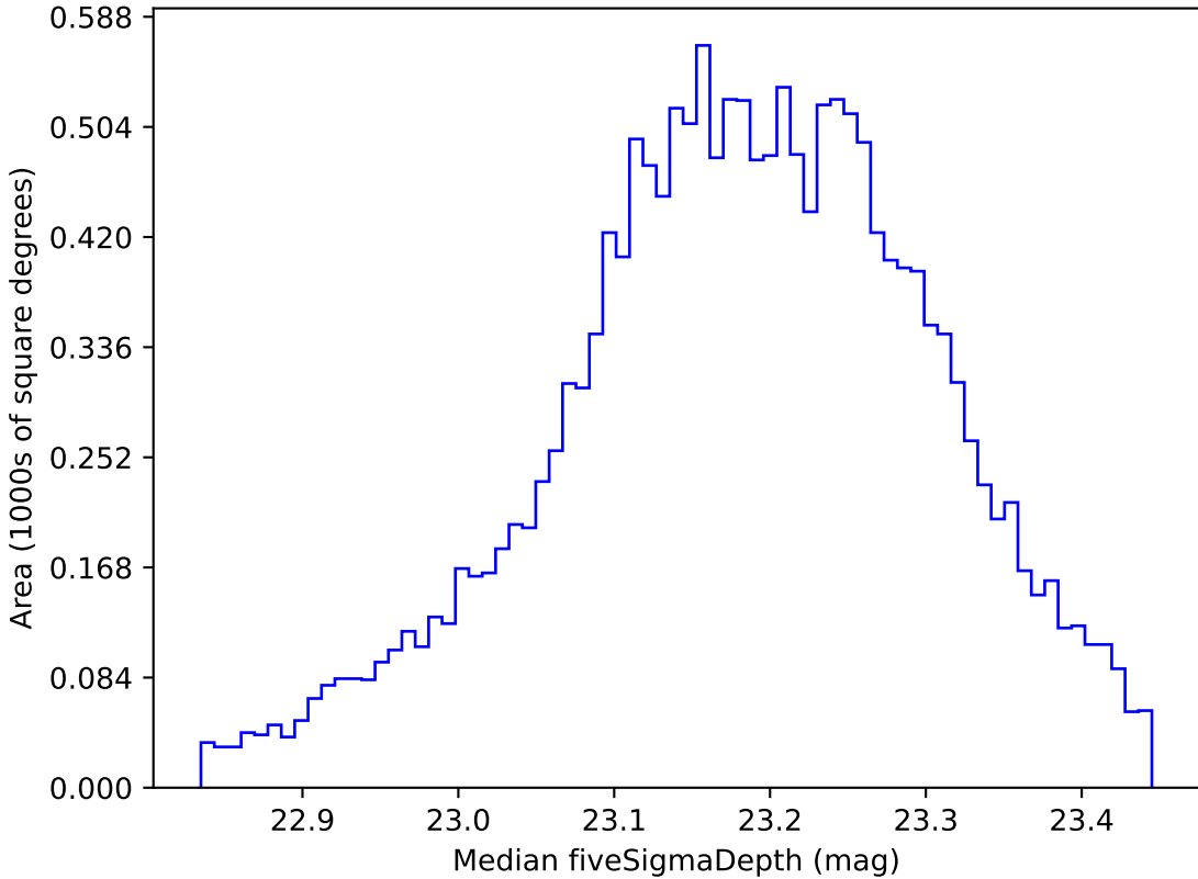
ddf_acor_sf15_lsf40_lsr20_v3.4_10yrs WFD u band: Median fiveSigmaDepth
