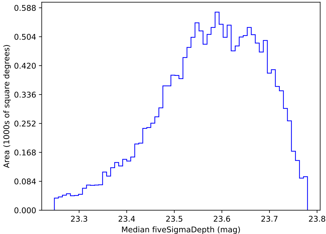
ddf_acor_sf15_lsf40_lsr20_v3.4_10yrs WFD i band: Median fiveSigmaDepth
