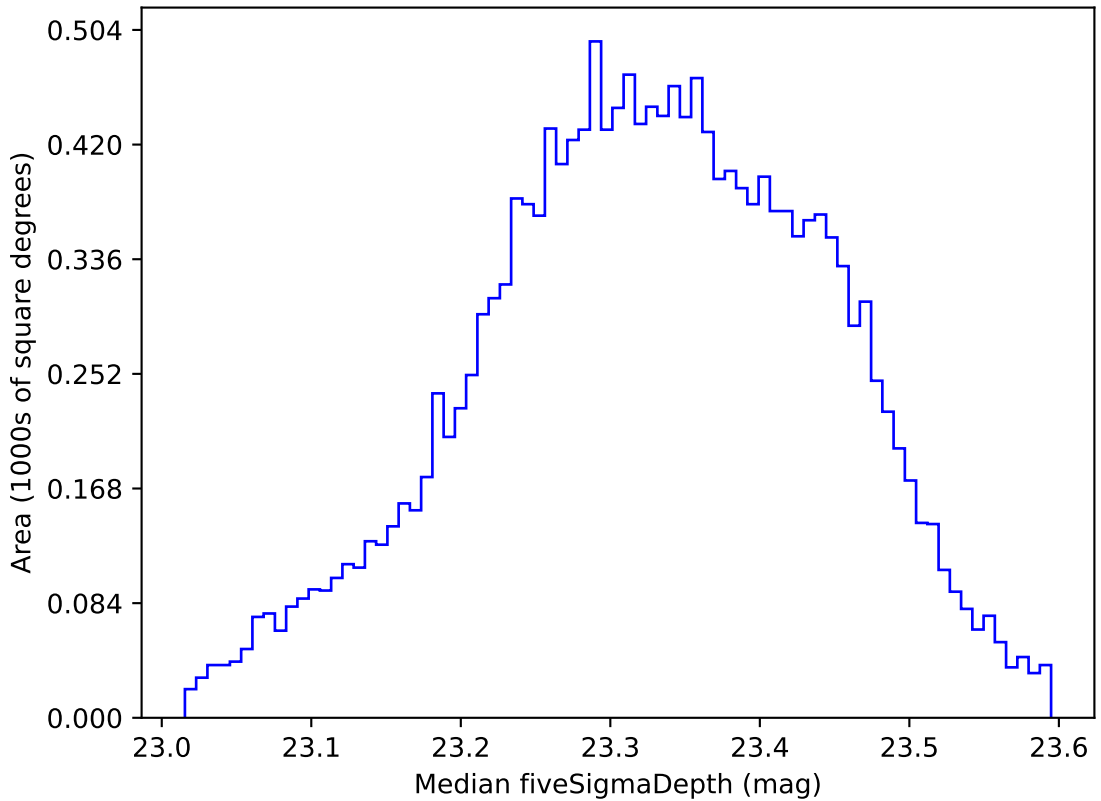
ddf_acor_sf15_lsf40_lsr20_v3.4_10yrs WFD all bands: Median fiveSigmaDepth
